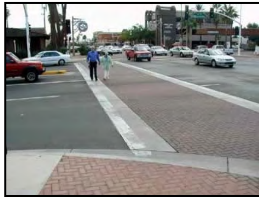
Exhibit 6-1: Textured Crosswalk
