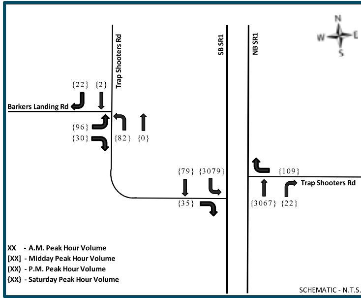
Figure 15 - 2028 Summer Saturday Peak Hour Turning Movement Traffic Volumes
