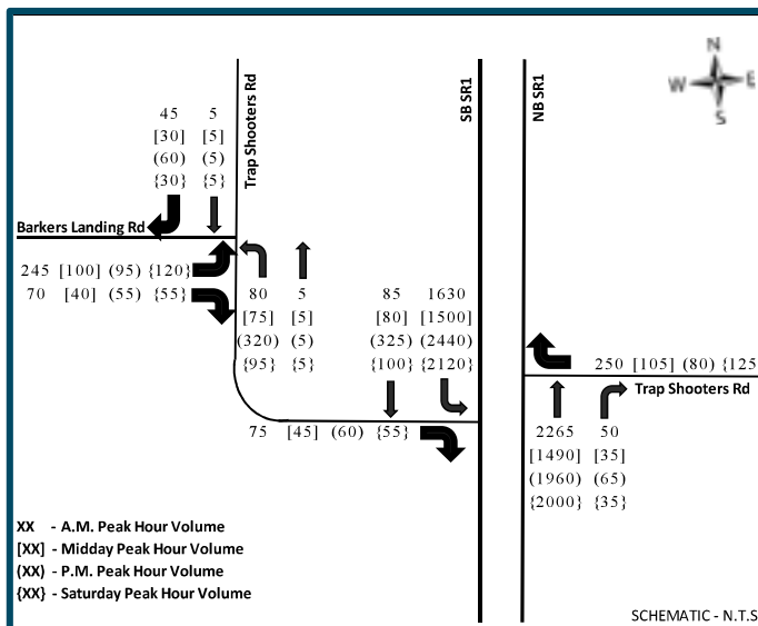
Figure 14- 2050 Non-Summer Peak Hour Turning Movement Traffic Volumes
