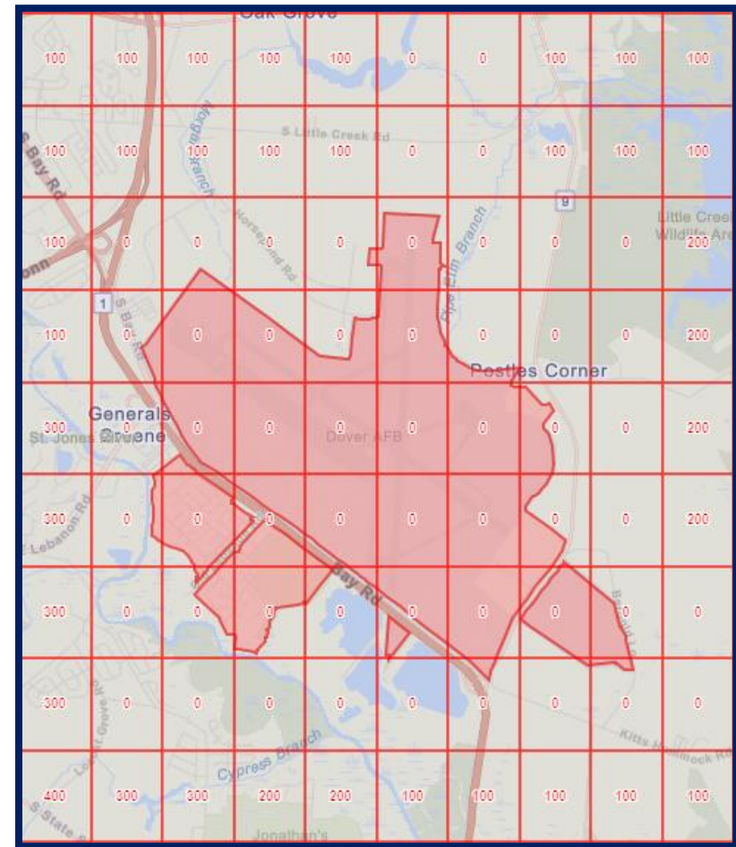
Figure 21 - UAS Restrictions and Height Limits
