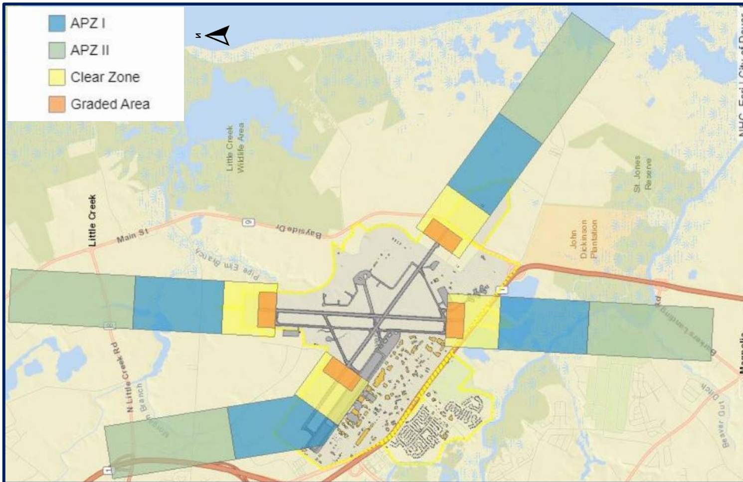
Figure 15 - DAFB Clear Zone and Accident Potential Zones
